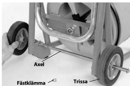
Figur 4 – Montera trissan
